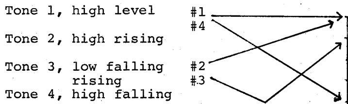
Figure 9: Chinese tones
